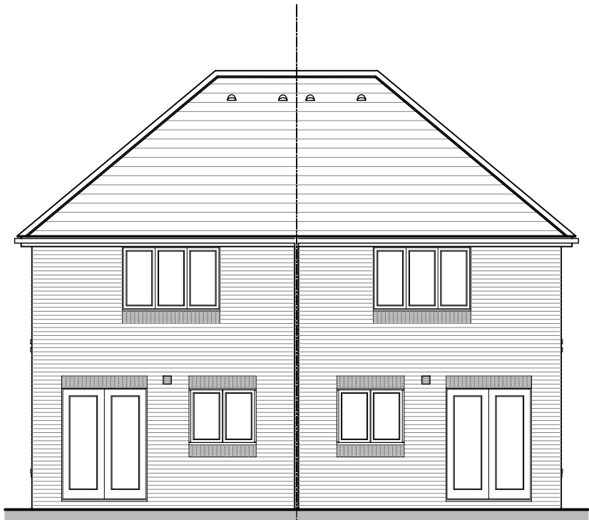
REAR ELEVATION (AS)
