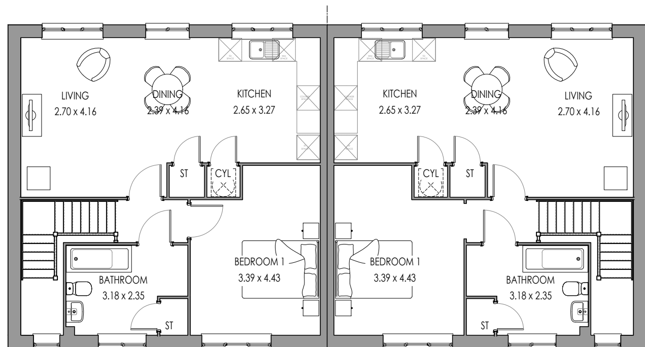
FIRST FLOOR (AS)
