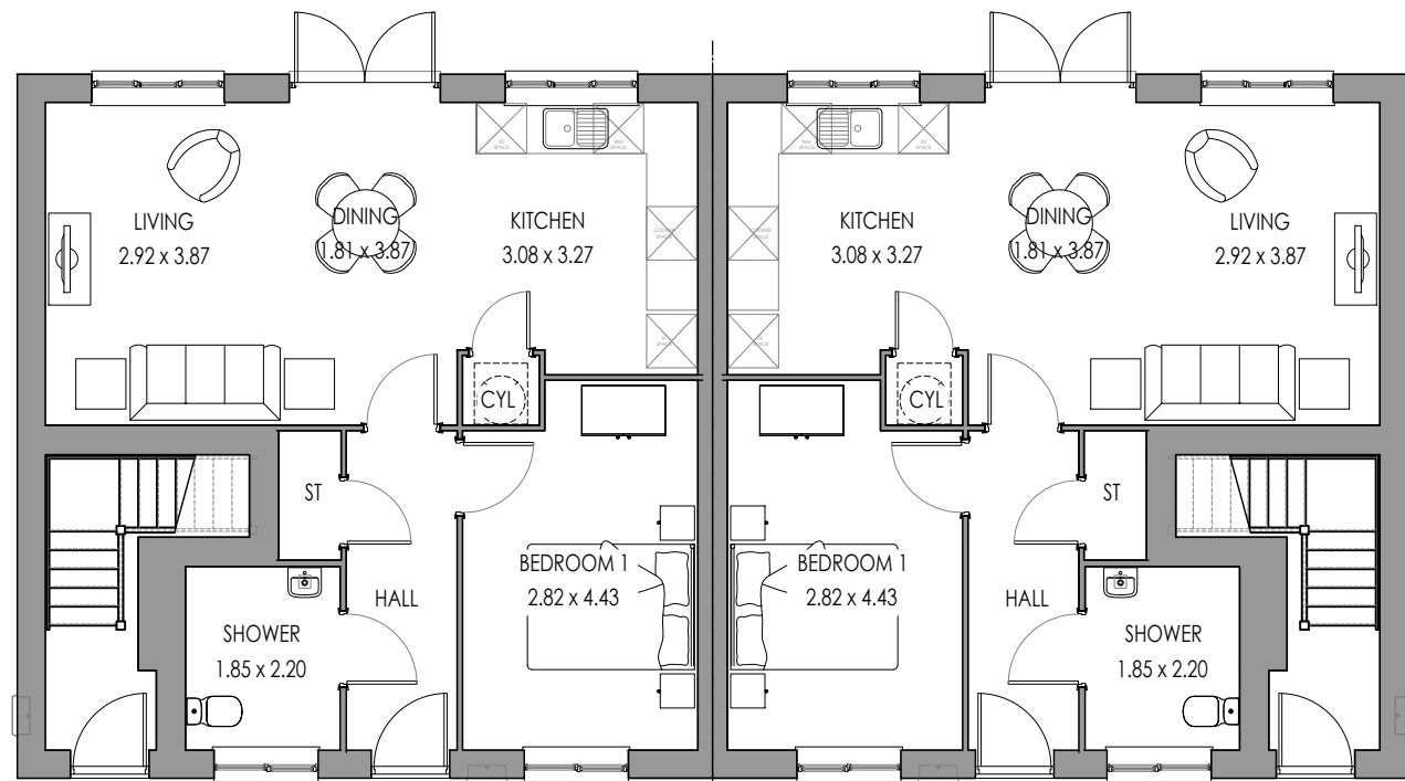
GROUND FLOOR (AS)
